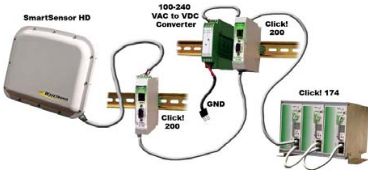
Figure 8 – Long cable run
