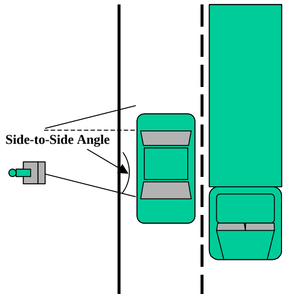
Figure 4 – Side-to-side positioning
