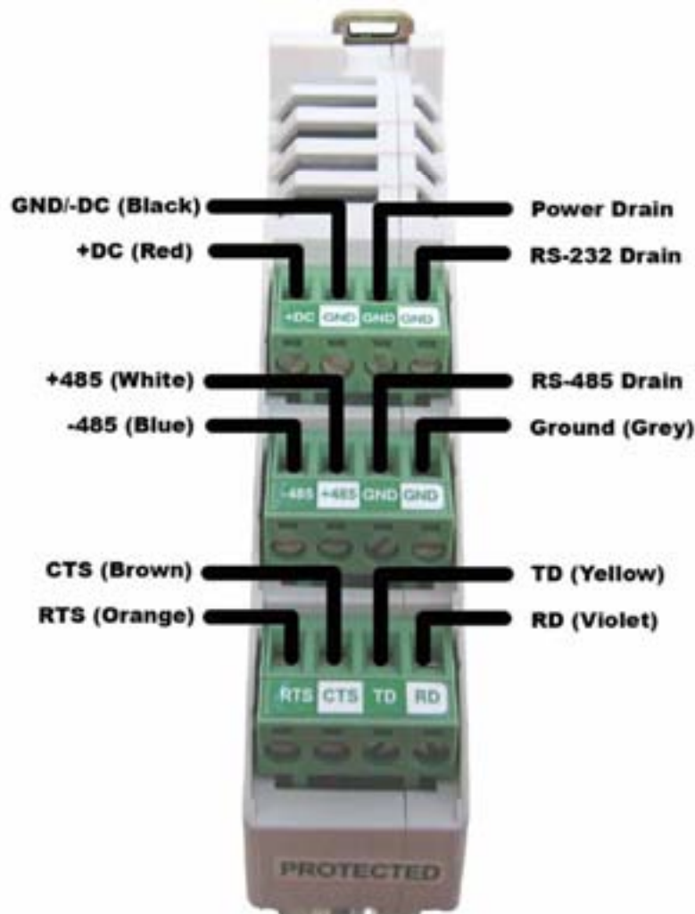
Figure 10 – Surge Protected Terminal Connections
