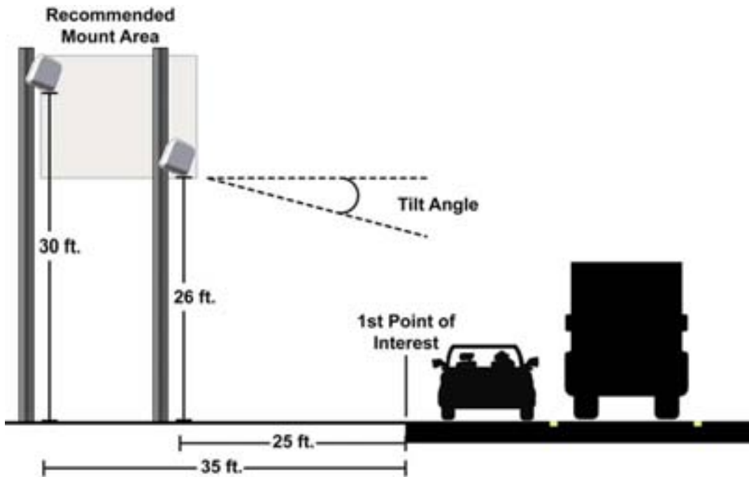
Figure 3 – Recommended Mounting Height
