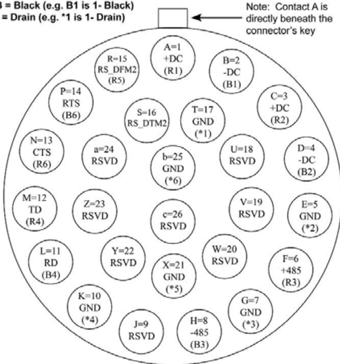
Figure 33 – Old SmartSensor SS105 Plug Connector Socket Assignment as seen from the solder cup side of the connector.
