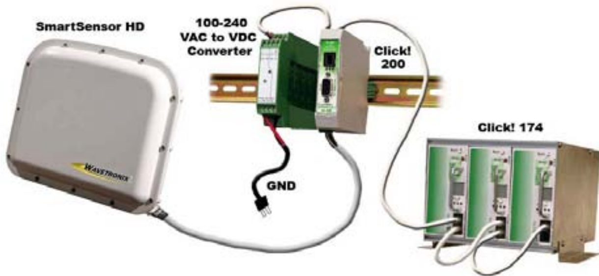
Figure 7 – Short cable run
