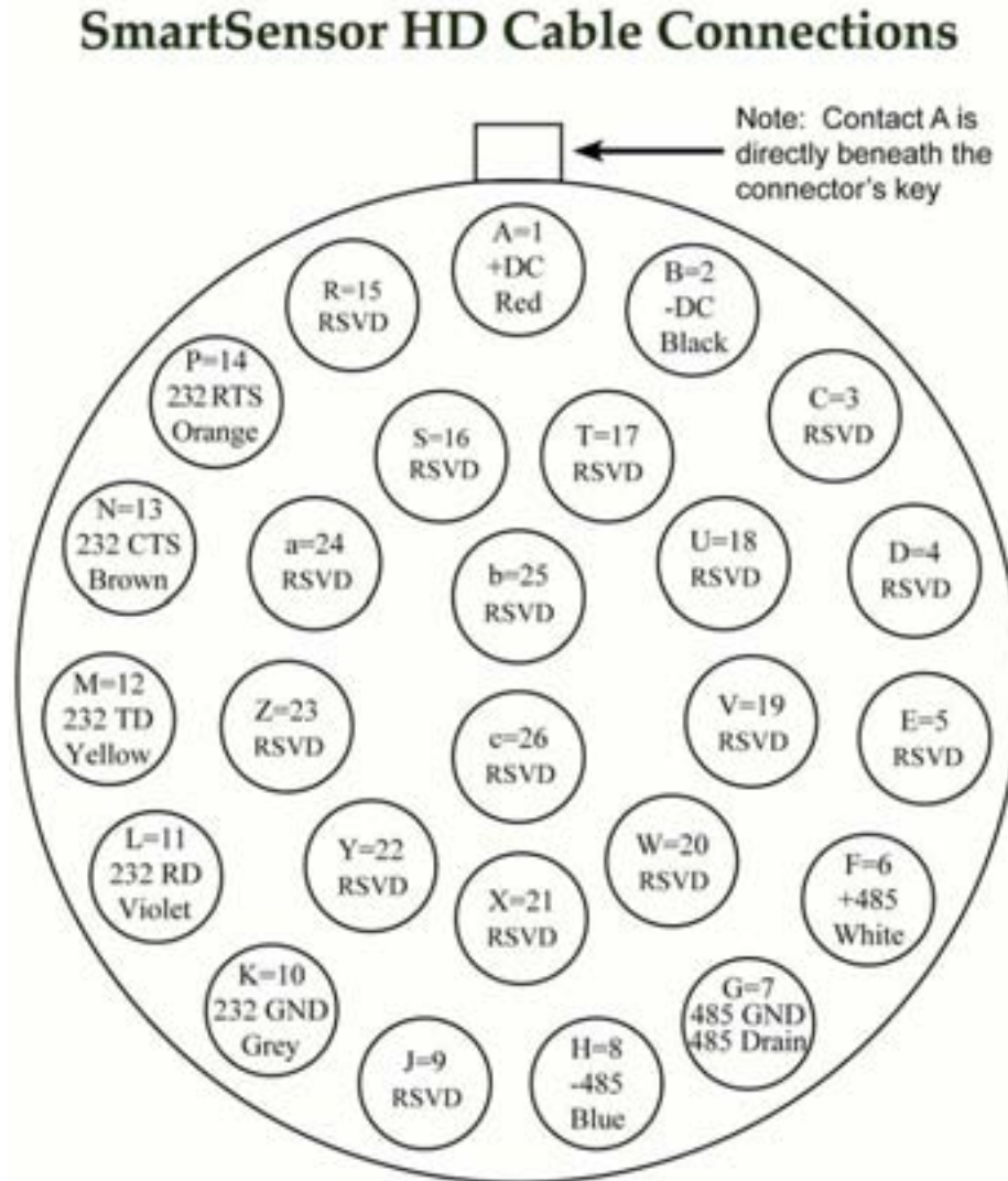
Figure 9 – SmartSensor HD SS125 Plug Connector Socket Assignment
