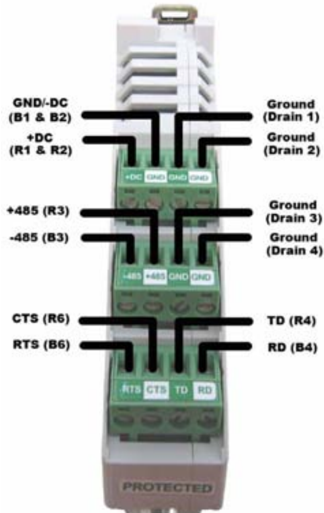
Figure 32 - Click! 200 Wiring (Old)
