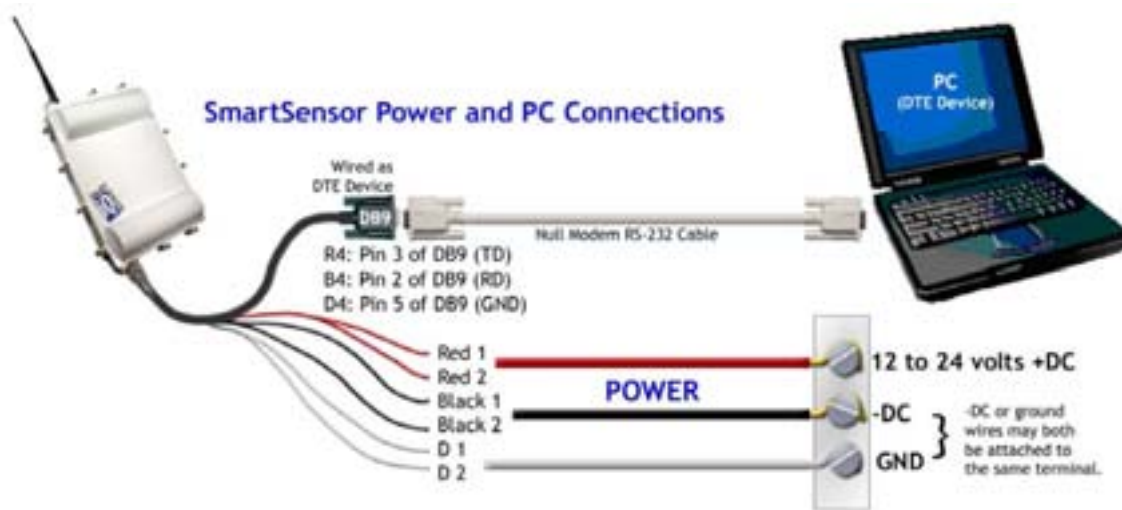
Figure 34 – Connecting a PC to the SmartSensor HD
