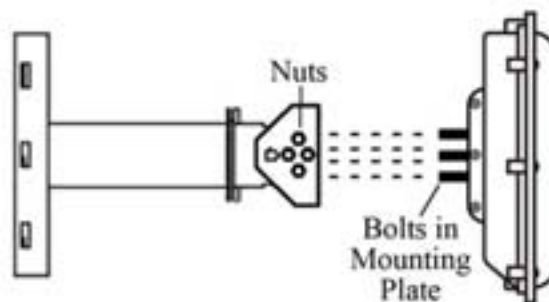
Figure 2 - Sensor Attachment
